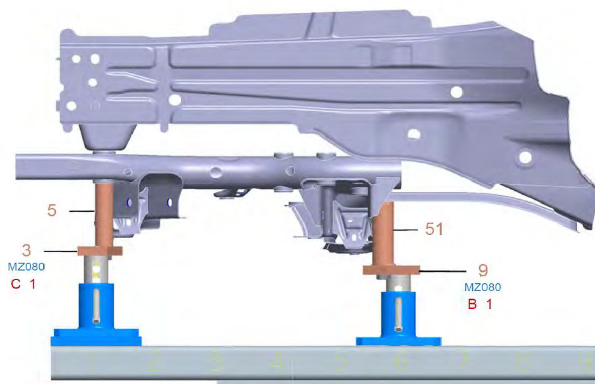
VERSION 2WD WITH BRACE
