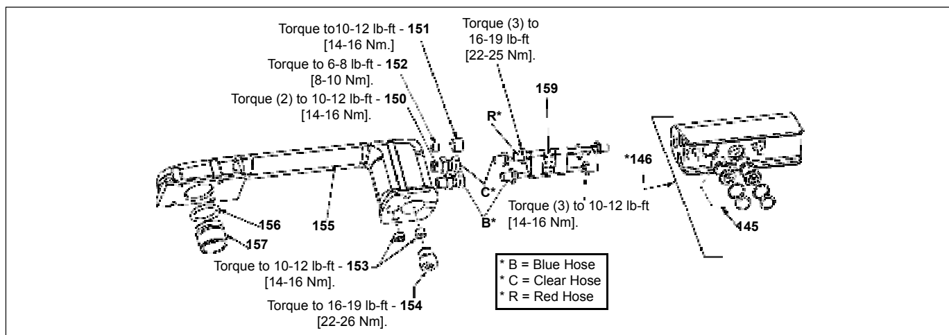
Figure 2b, Pendant Handle Assembly
